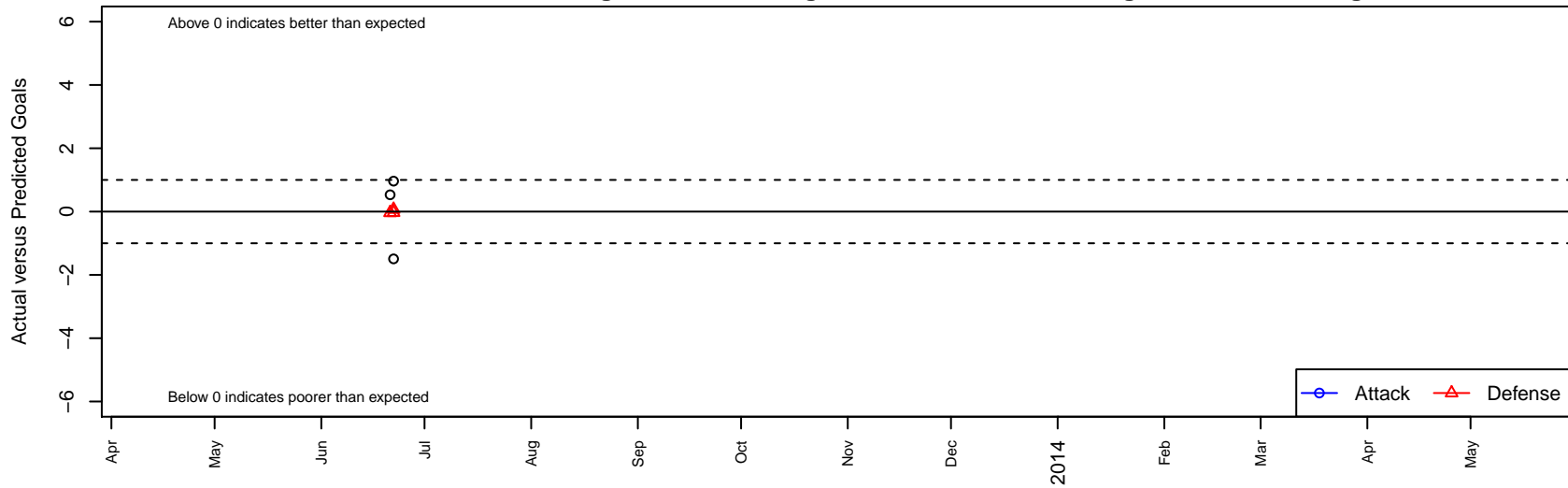
Lakehill Gold B96 Dots are actual minus expected GF (blue circles) and GA (red triangles). Blue line is smoothed change in attack strength. Red is smoothed change in defense strength.
